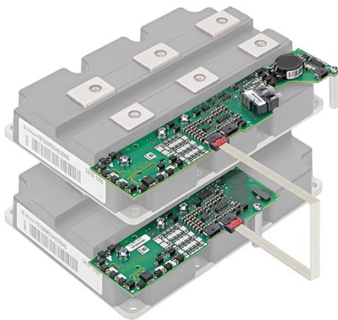
Fig. 1 1SP0635 Driver Plug-and-Play Master + Slave
